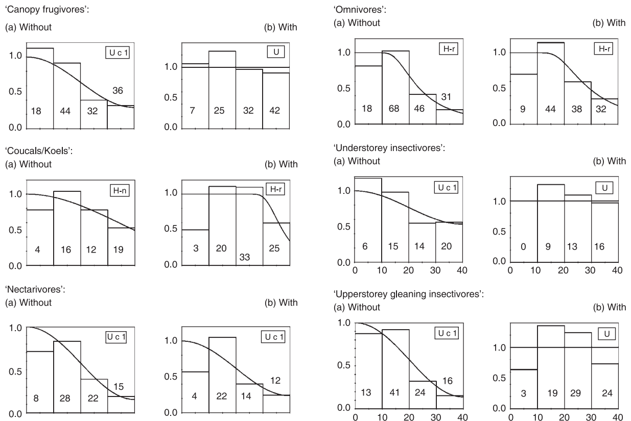
Figure 3. Detection function plots over 40 m from point transects with (a) no settling down period (Without) and (b) a 10-min settling down period (With). Radial distance ( x -axis) is grouped into four 10-m detection intervals (0–10, 11–20, 21–30 and 31–40 m). Bars represent count frequencies scaled (divided) by detection distance. Count frequencies are indicated in each 10-m bar. The curves signify the fitted detection model (probability of detection = 1.0 at 0 m). The key function (U – Uniform, H-n – Half-normal, H-r – Hazard-rate) and series adjustment term (c – cosine, number of terms = 1) of the detection model are displayed in the top right corner of each figure.
